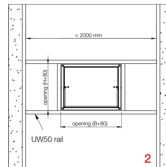
E-FD-MF2 Fire damper installation in 90 mm Shaft wall without metal studs ( < 2000 mm)
