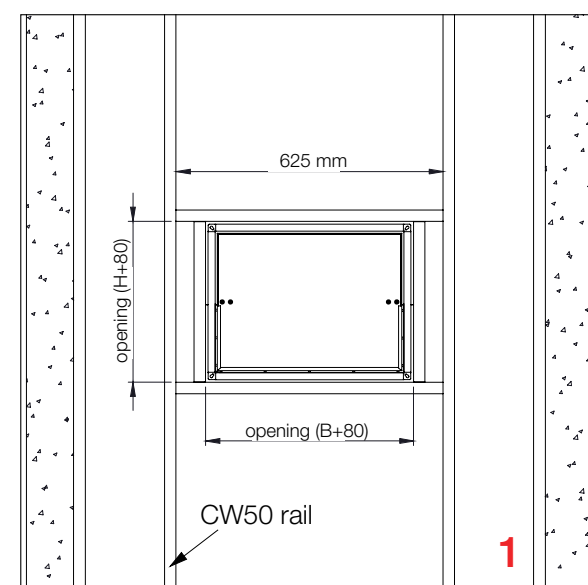
E-FD-MF2 Fire damper ( B < 625 mm) installation in 90 mm shaft wall with metal studs
