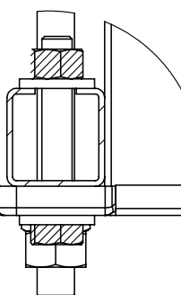
Detail A
