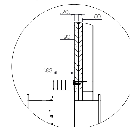
E-FD25, E-FD40 - side cross section
