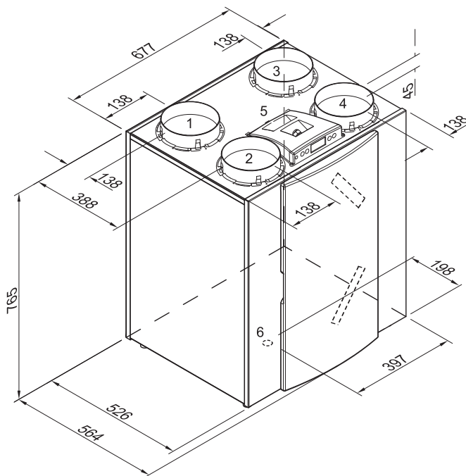
Ubiflux Right-handed 4/0
