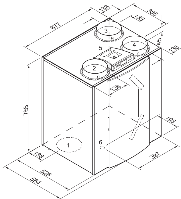
Ubiflux Right-handed 3/1
