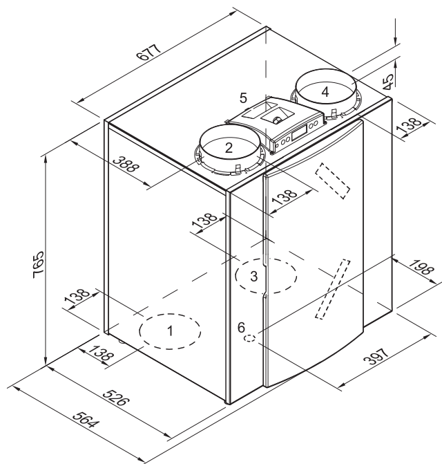
Ubiflux Right-handed 2/2
